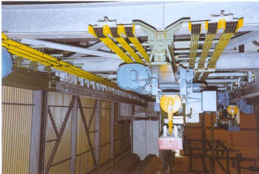
Automatic crane installation for transfer operation with pick up guides in a zinc coating plant.
