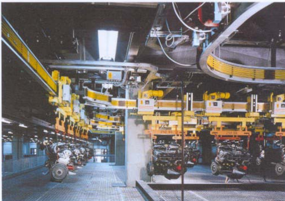
Back-up line installation of an electrically driven trolley conveyor for the transport of motors.
